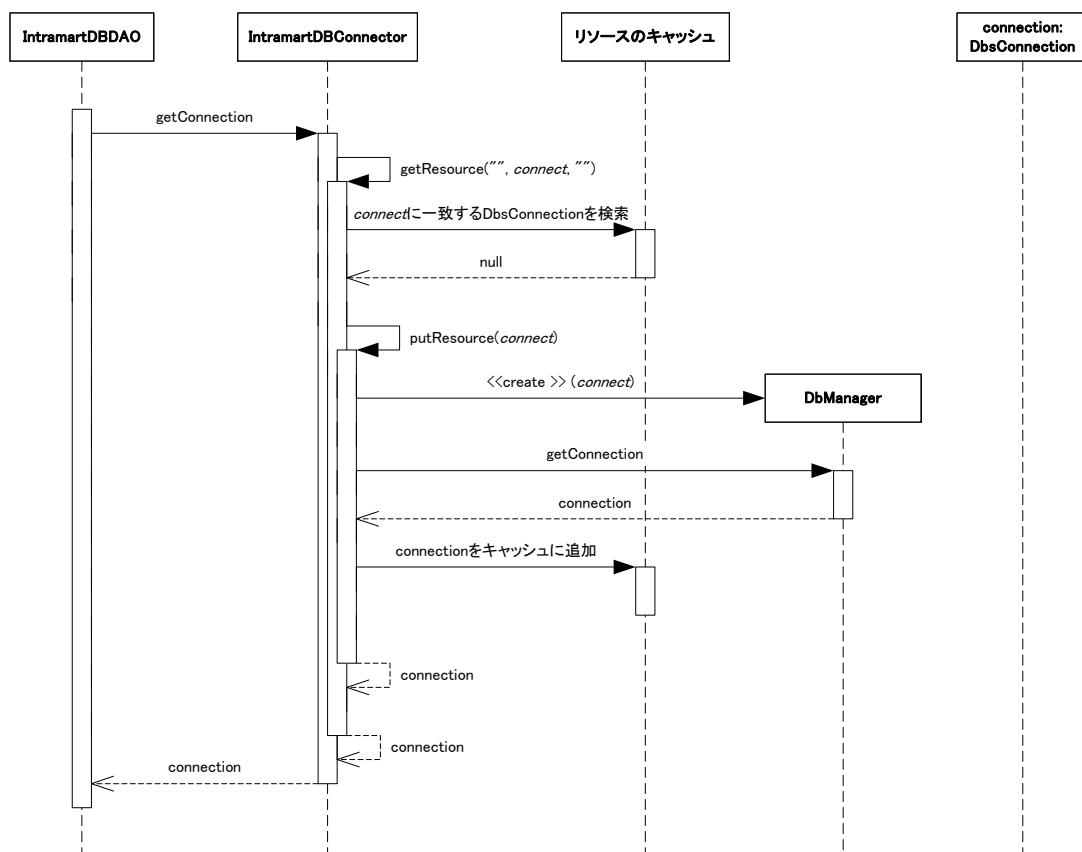
図 5-35 Connection の取得 (IntramartDBConnector)
